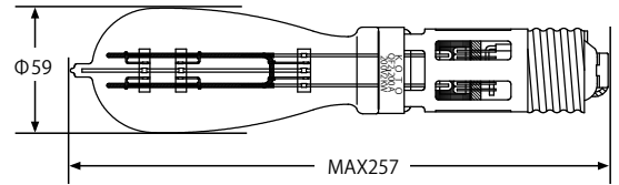
QF2-200A
